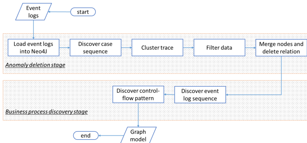
Figure 1. From event logs to generated anomalous-free business process model in the form of a graph model
