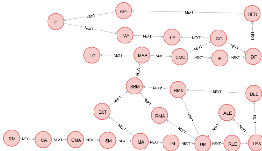
Figure 1. Filtered graph model with sequence relation
