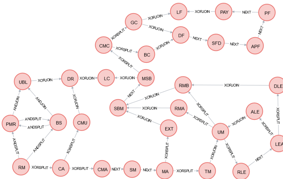
Figure 3. Unfiltered graph model with a control-flow pattern
