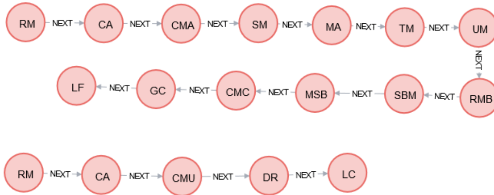
Figure 9. Data loading and case sequence discovery limited on PP1 and PP2 case IDs
